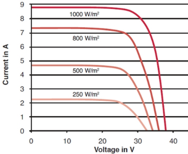
I-U characteristic curve at 1000-800-500-250 W/m 2
